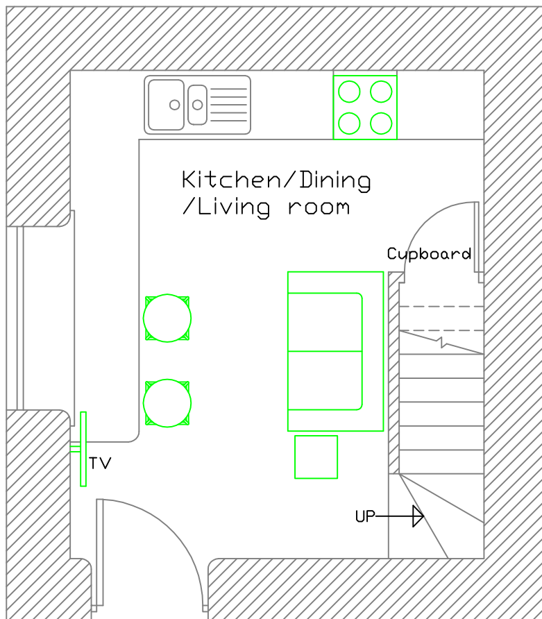
The Dairy Ground floor plan
